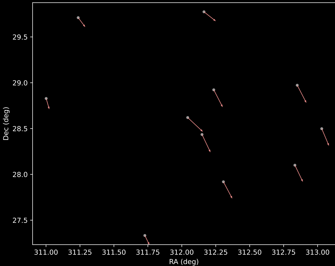
APOGEE DR17 Cluster 7 Proper Motion Vectors (n=11)
