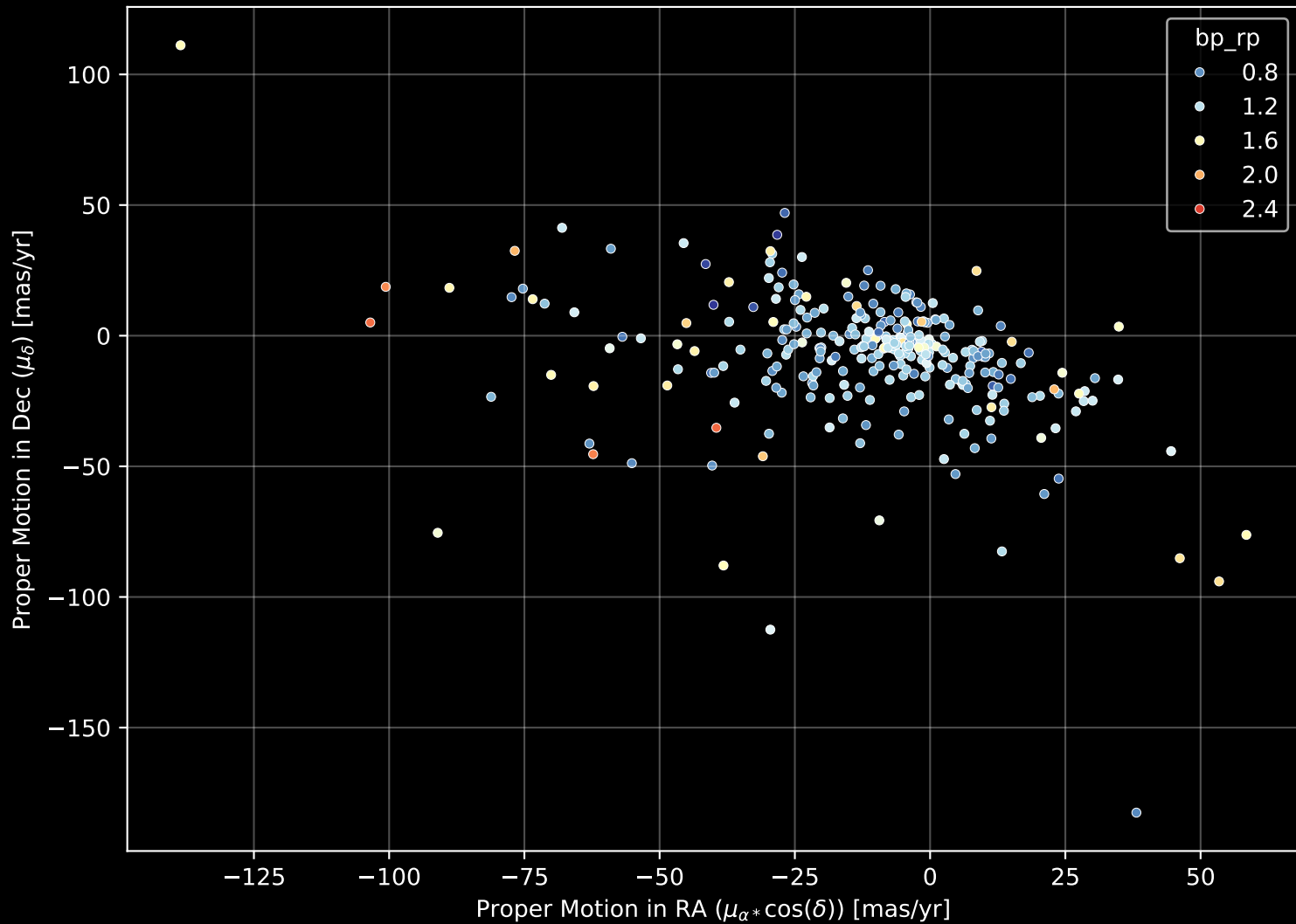
APOGEE DR17 Field: [N5466] Proper Motion Diagram (n= 309)
