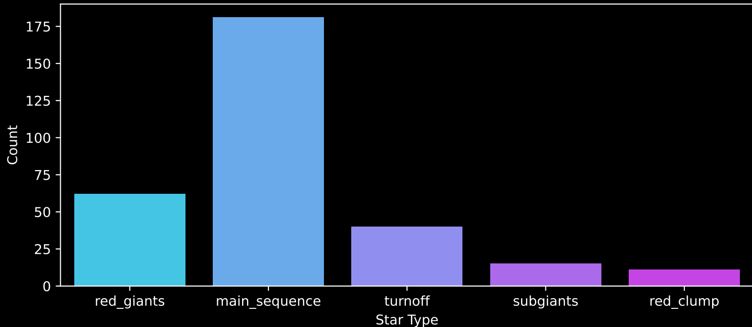
APOGEE DR17 Field: [N5466] Count plot of Star Type
