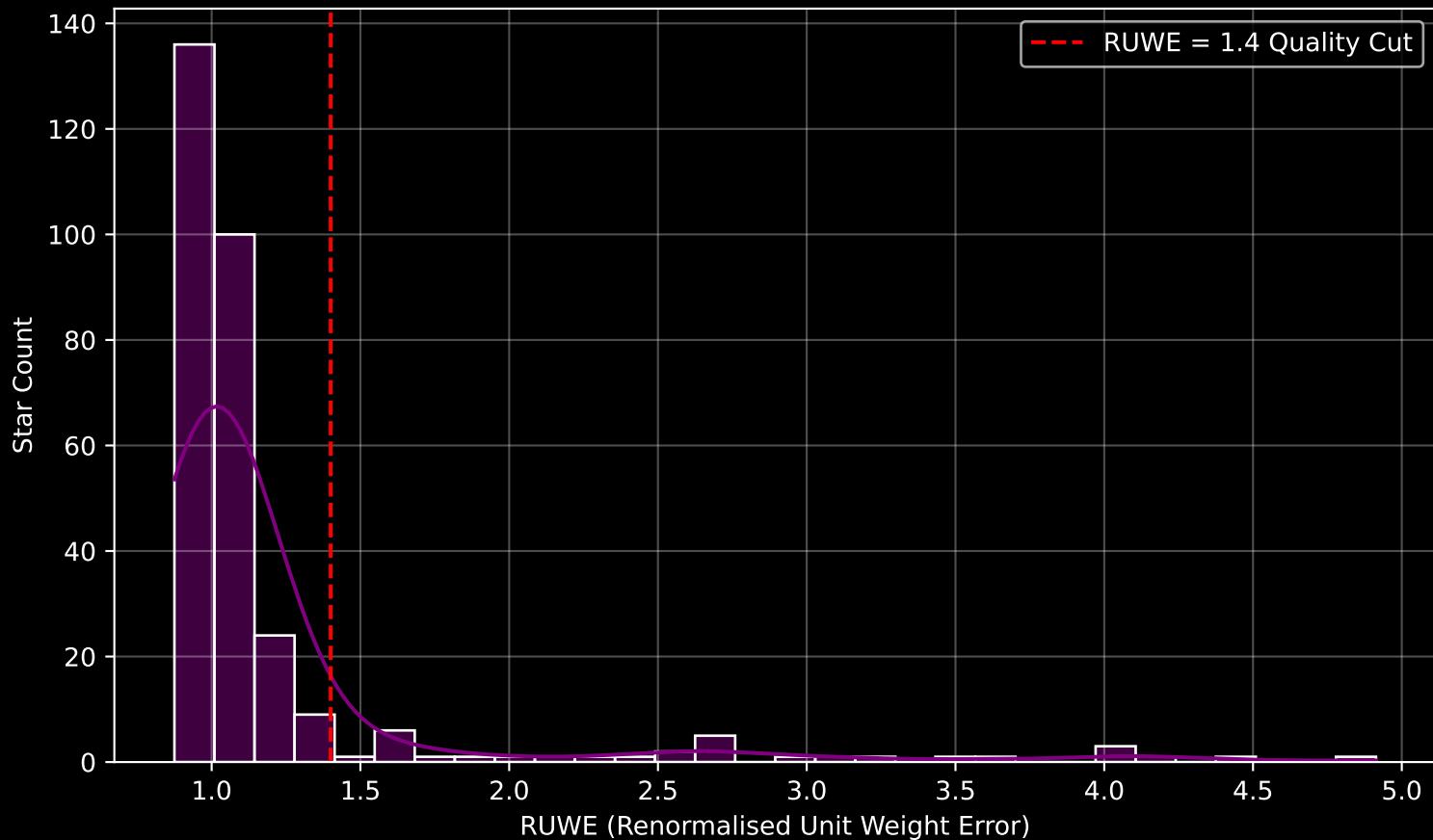
GAPOGEE DR17 Field [N5466] RUWE Distribution (n= 300)
