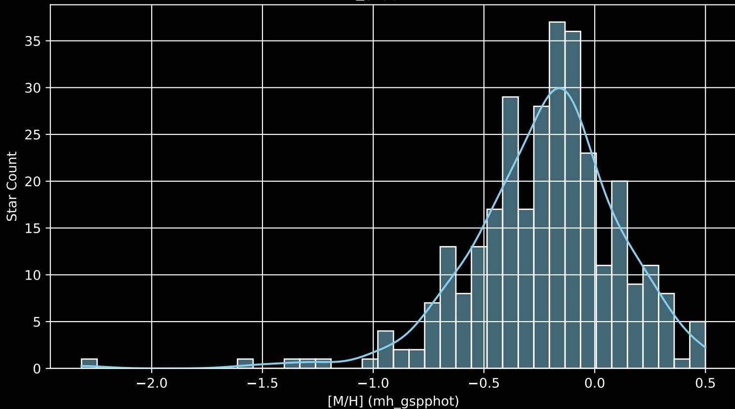
APOGEE DR17 Field: [N5466 [M/H] (mh_gspphot) (n= 307)
