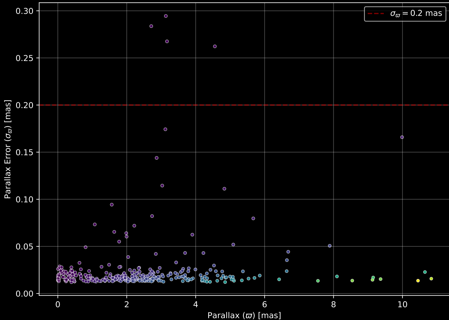
APOGEE DR17 Field: [N5466] Parallax Quality (n= 309)
